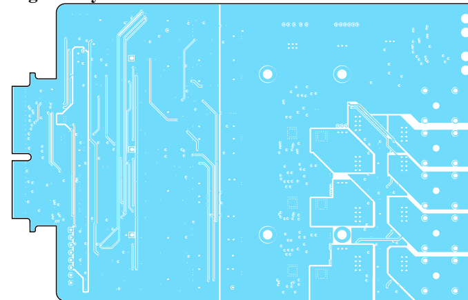
Ground and Power Planes
